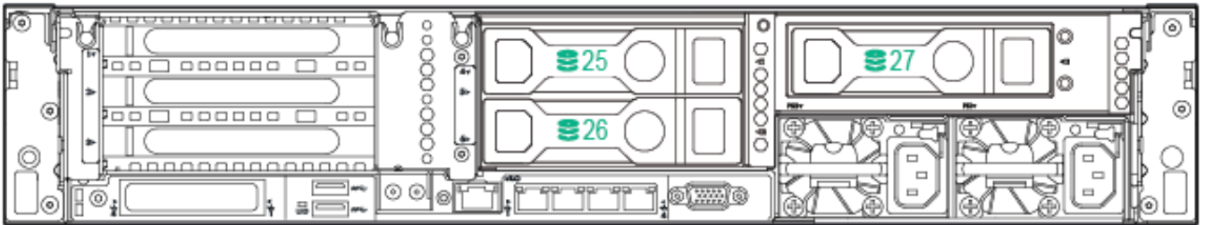
12 LFF + 3 rear LFF hot-plug drive model
